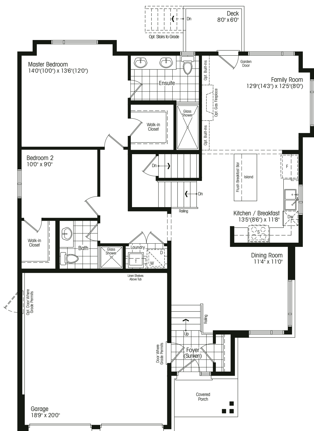
Main Floor Elev. A
