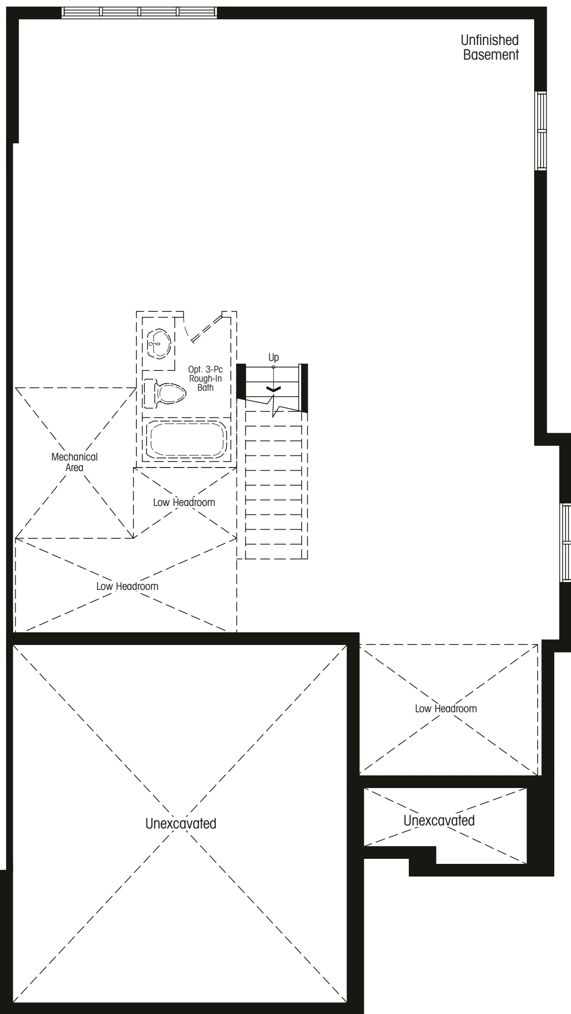
Basement Elev. A
